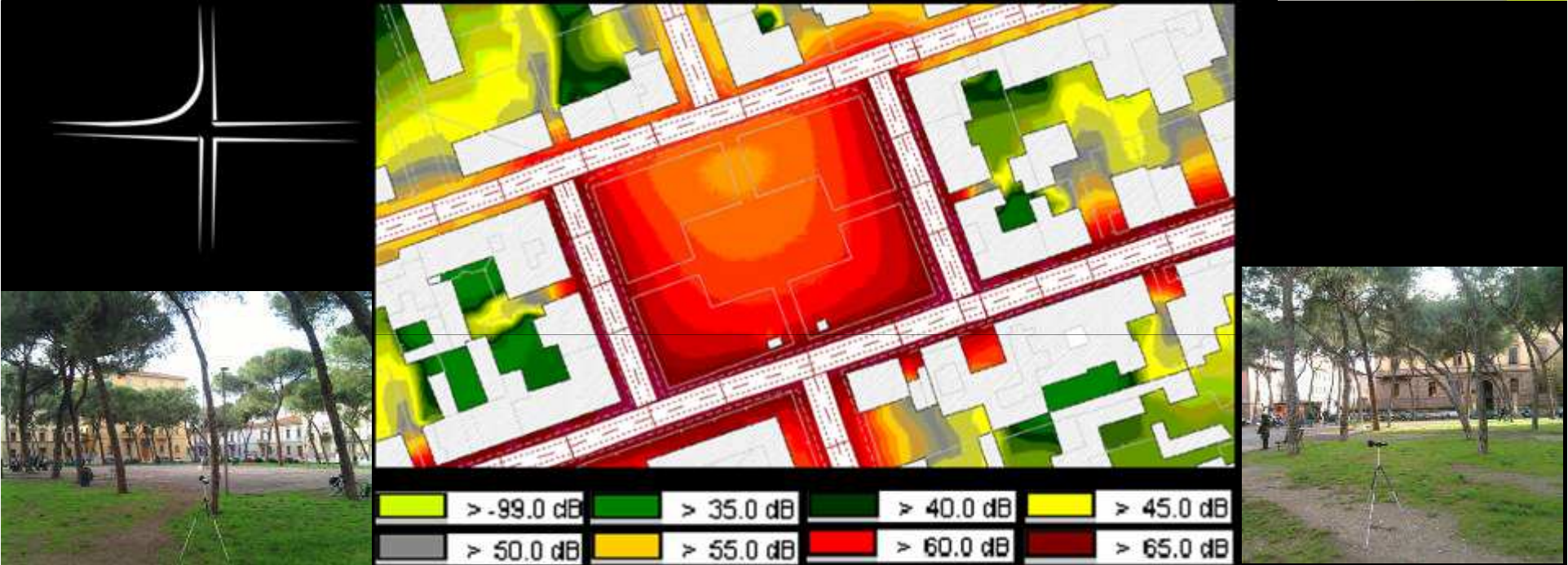
ACOUSTIC MAP: study of the noise propagation caused by the road
